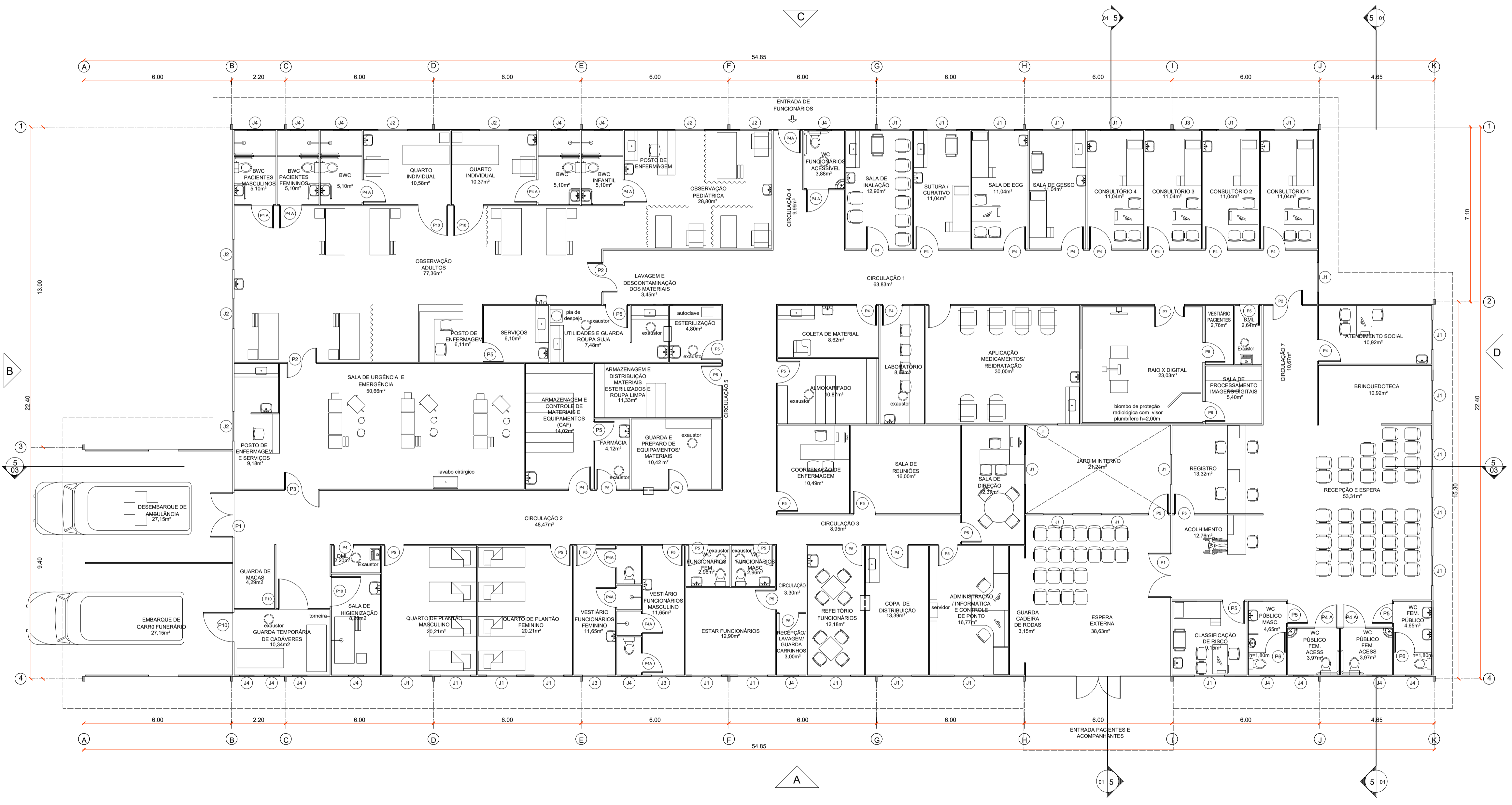
1 LAYOUT ESC: 1/100
